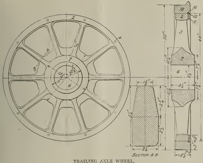
TRAILING AXLE WHEEL.
